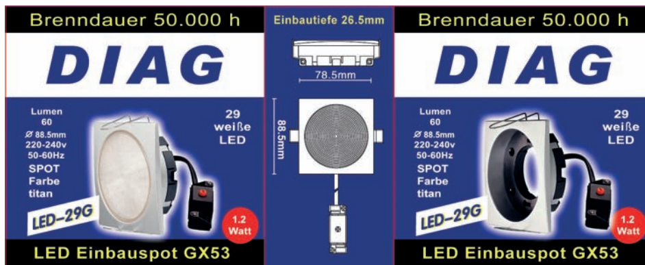
DI 10287 Einbauset / In-ground-set Titan / titanium, quadratisch / quadratic 29x LED GX53/230V/1,2W; weiß / white 88,5x88,5mm, Tiefe / depth 26,5mm
