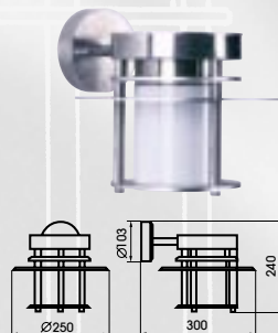
AL 690601 IP 44, A 60, max. 75 W, E 27 Opal glas
