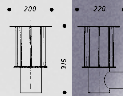
AL 690686 IP 44, A 60, max. 75 W, E 27 Opal glas
