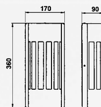
AL 696010 IP 44, A 60, max. 75 W, E 27 Opal glas
