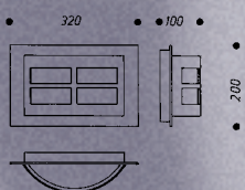
AL 696091 IP 44, A 60, max. 75 W, E 27 Opal glas
