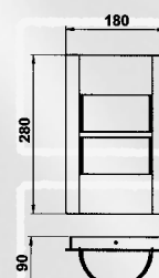
AL 696109 IP 44, A 60, max. 75 W, E 27 Opal glas
