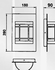
AL 696097 IP 44, A 60, max. 75 W, E 27 Opal glas
