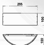
AL 696142 IP 44, QT-DE 60 W, R7s Opal glas
