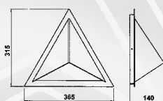
AL 696123 IP 44, A 60, max. 75 W, E 27 Opal glas
